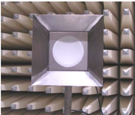
Fig. 3 measurement SXTG 5HPacD-SA (anechoic hall VUS B.Bystrica, Slovakia )
