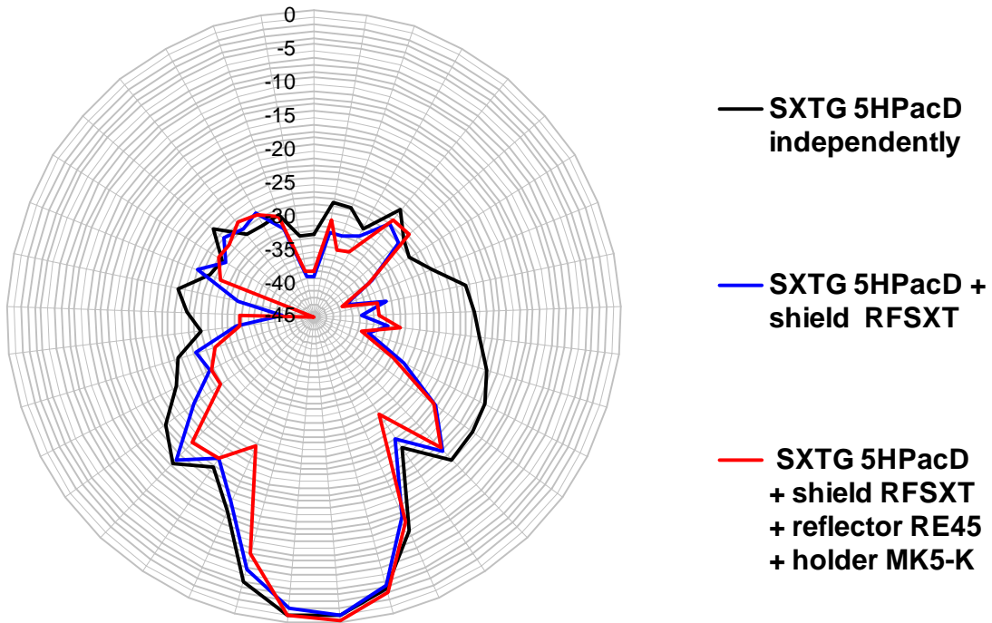
Radiation pattern envelope (RPE) V - polarization
