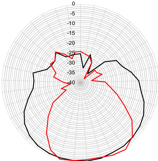
Radiation pattern envelope (RPE) V - polarization
