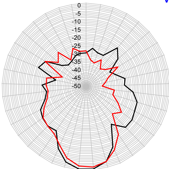
Radiation pattern envelope (RPE) V - polarization
